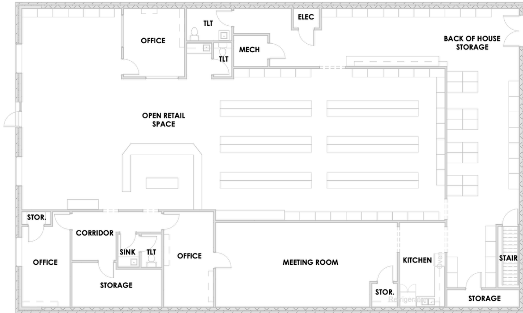
1 MAIN LEVEL FLOOR PLAN 3/32" = 1'-0"
