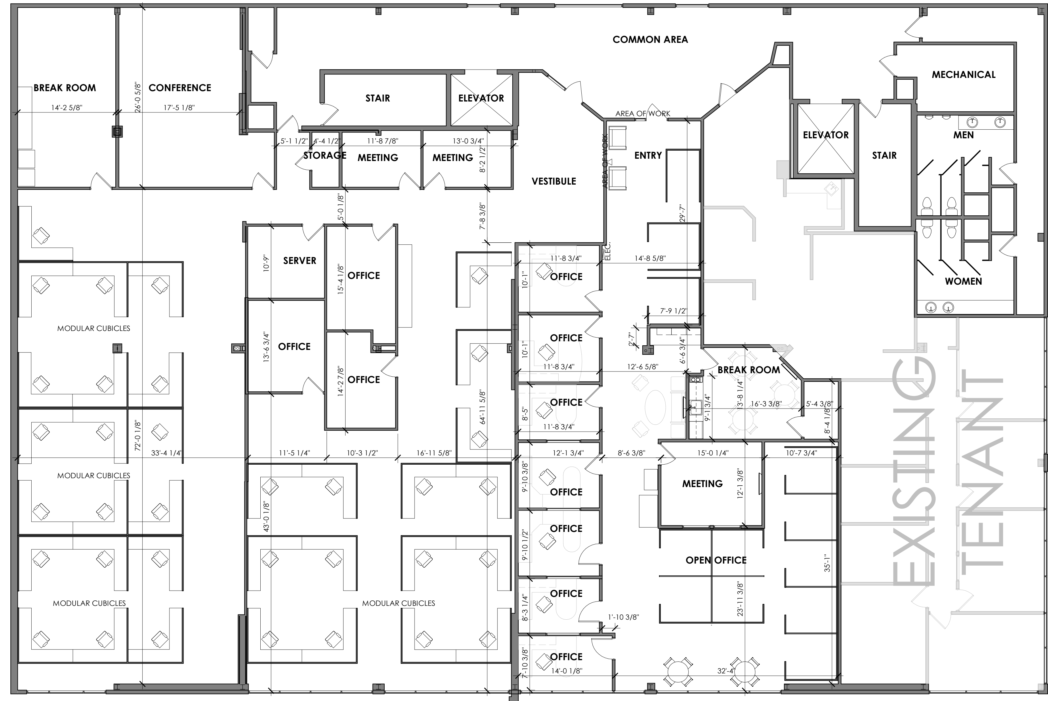
① REMODEL PLAN 1/8" = 1'-0"
