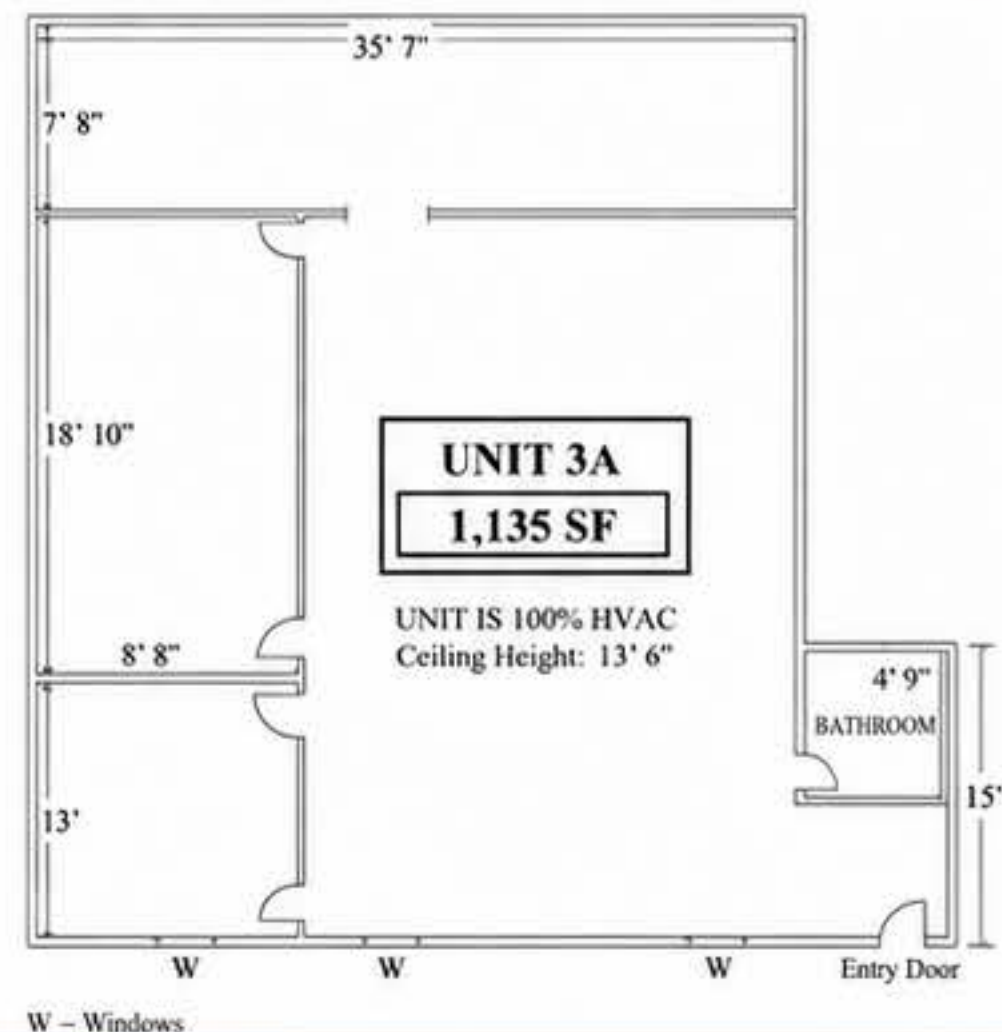
UNIT 3A FLOOR PLAN
