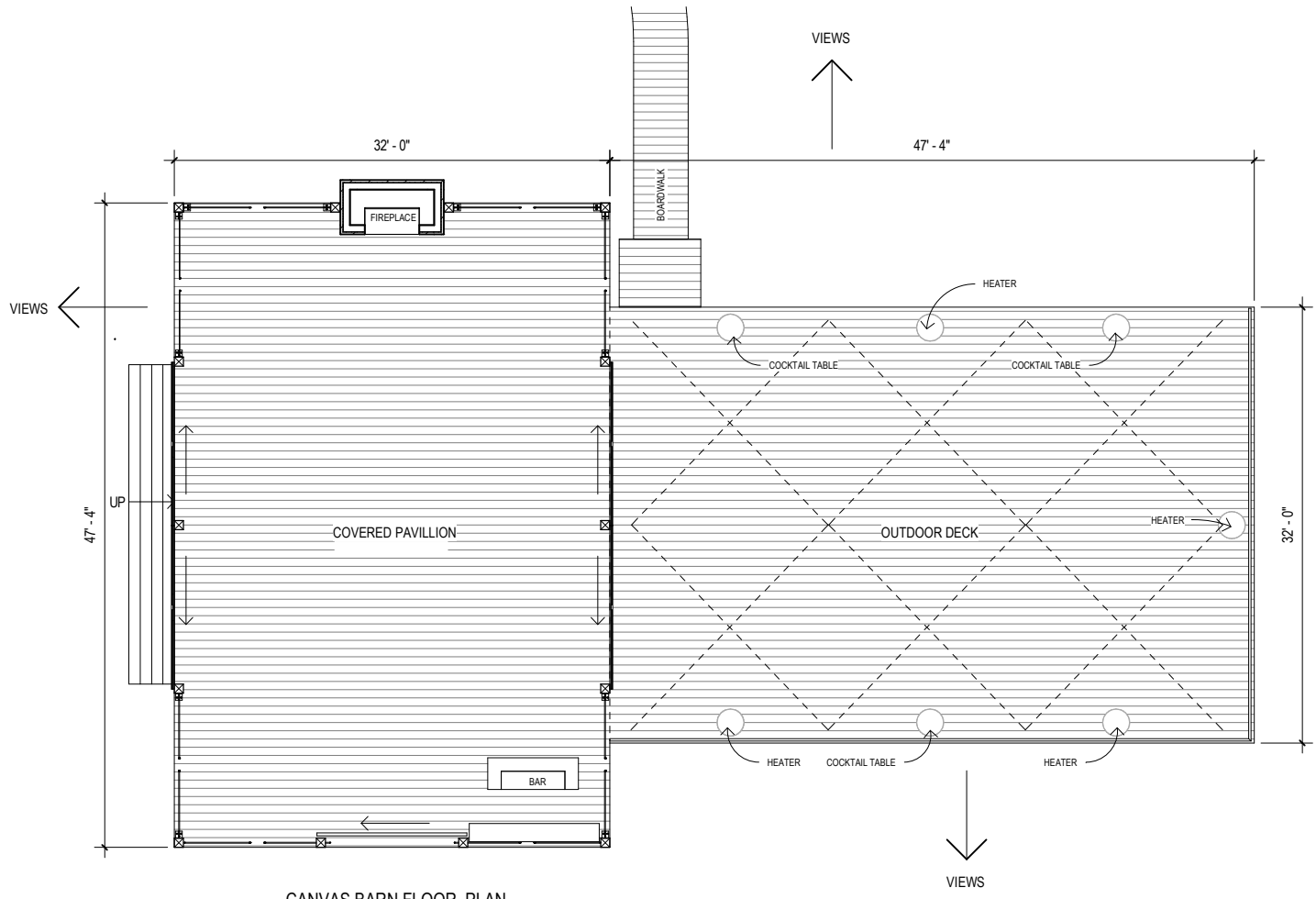
CANVAS BARN FLOOR PLAN
