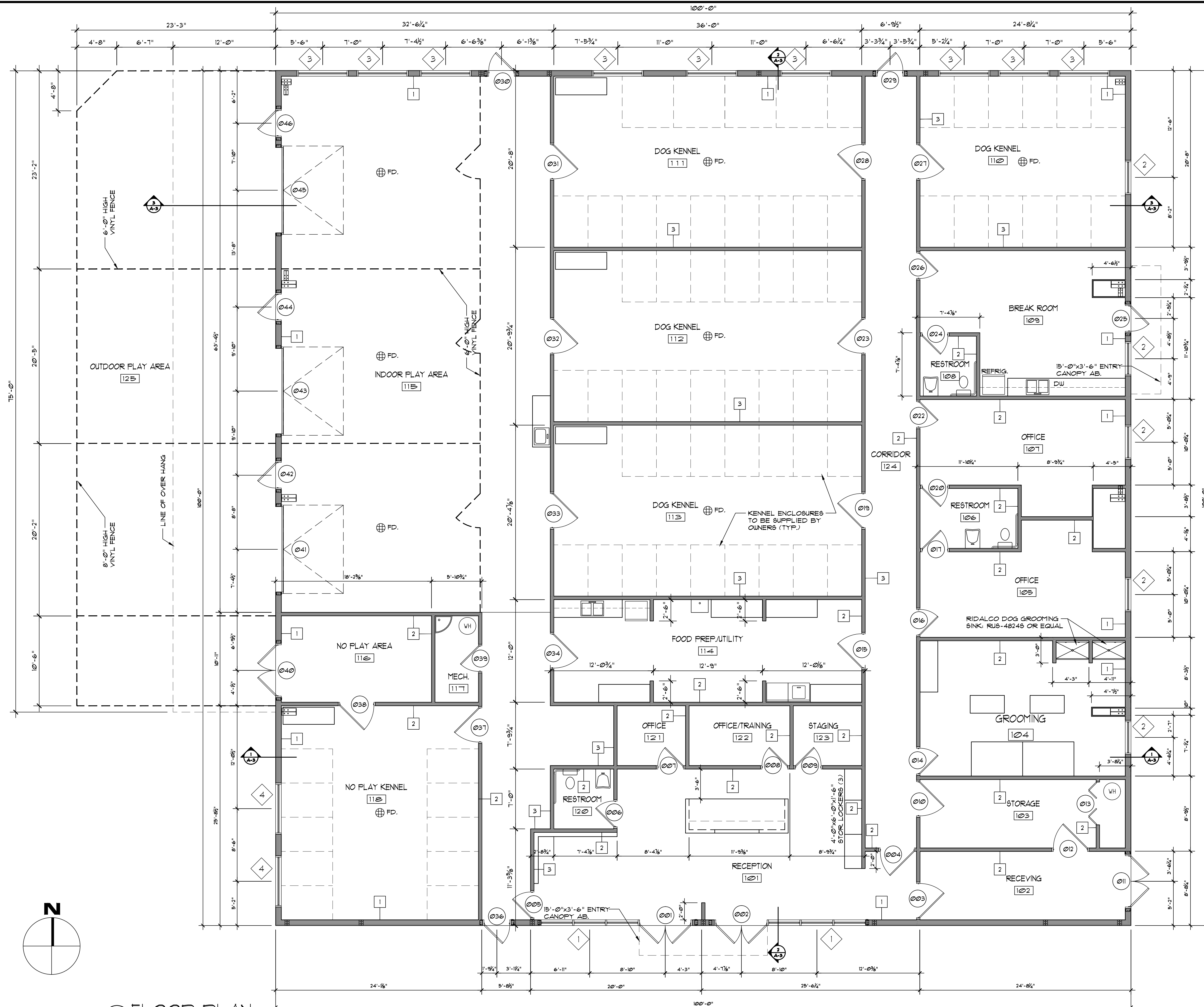
1 FLOOR PLAN 3/16" = 1'-0"
