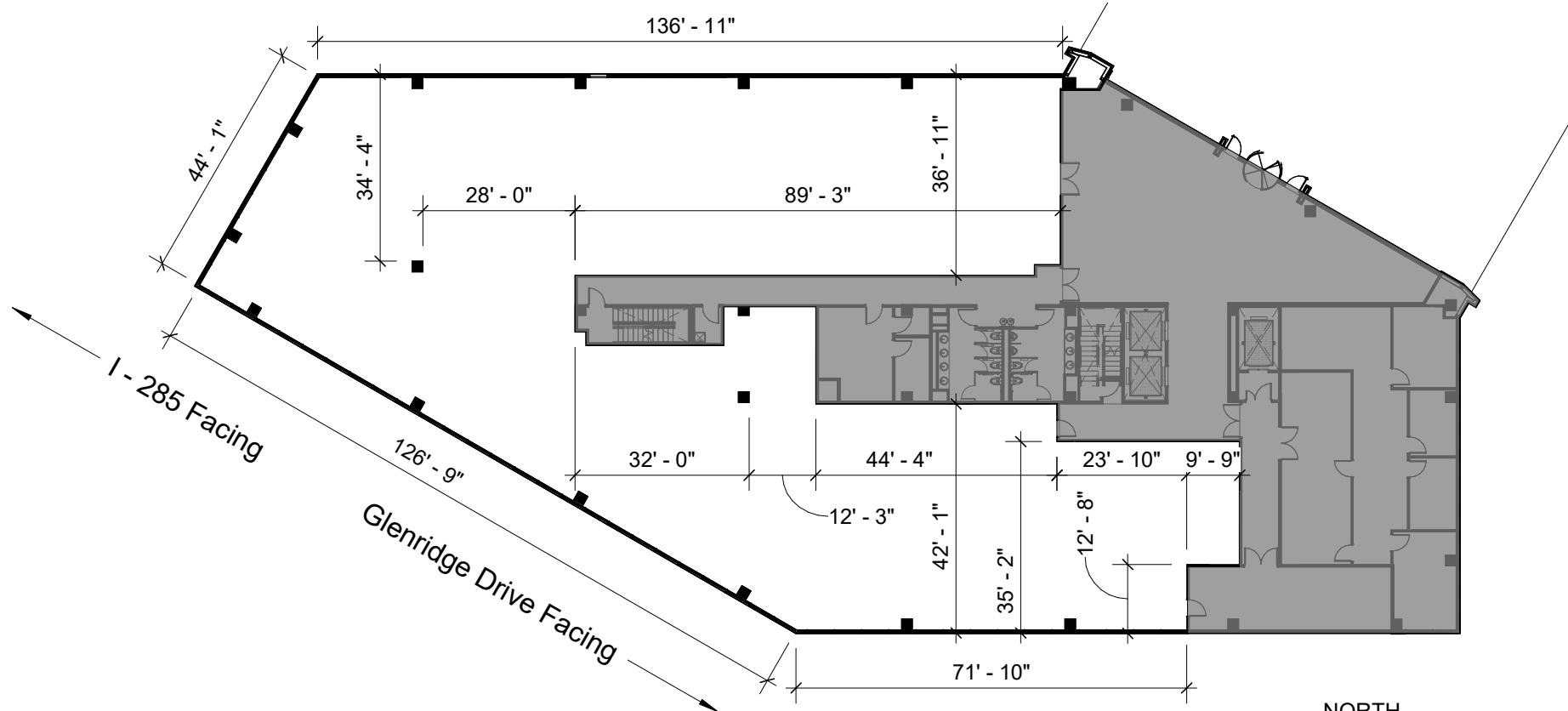
Floor Plan - Suite 100 West
