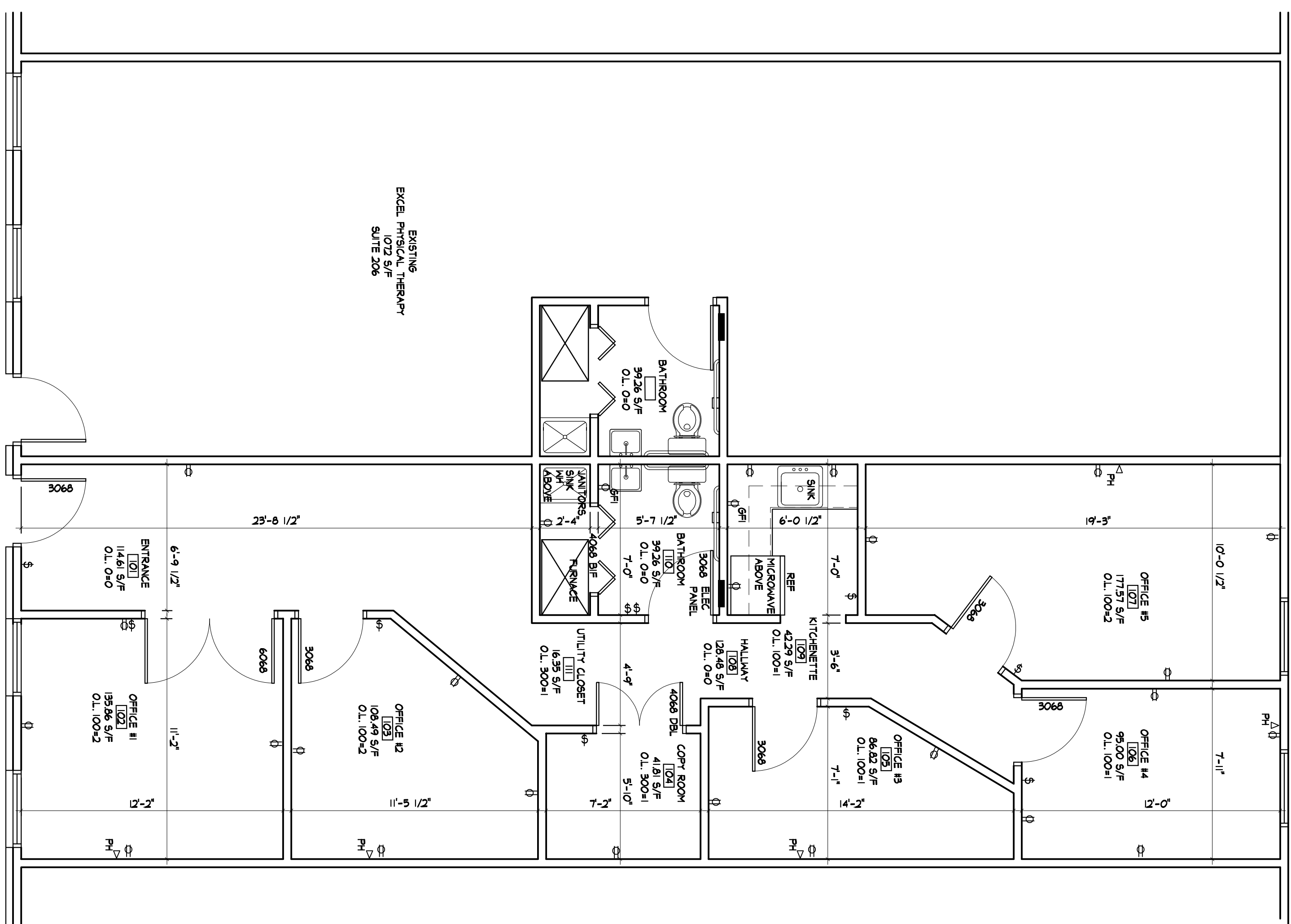
AS-BUILT FLOOR PLAN SCALE: 1/4" = 1'-0"
