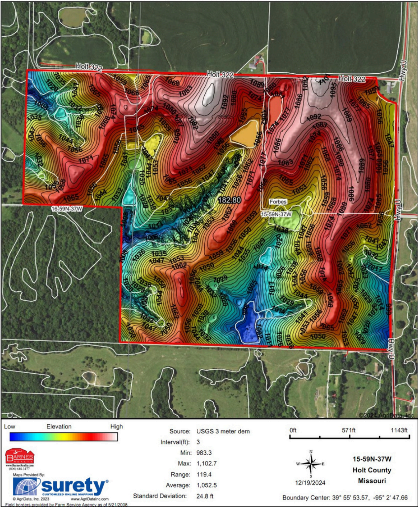
Topography Hillshade
