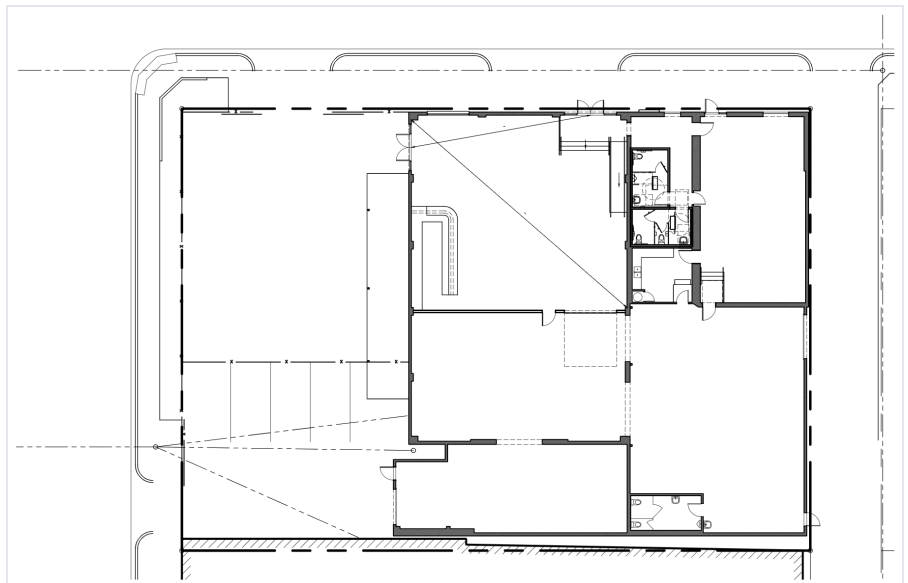
FLOOR PLAN
