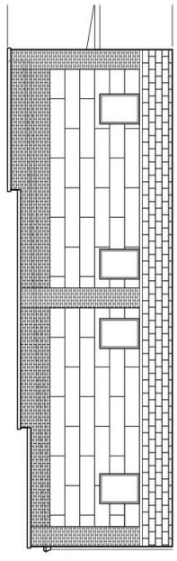
4 Left Elevation 3/16" = 1'-0"
