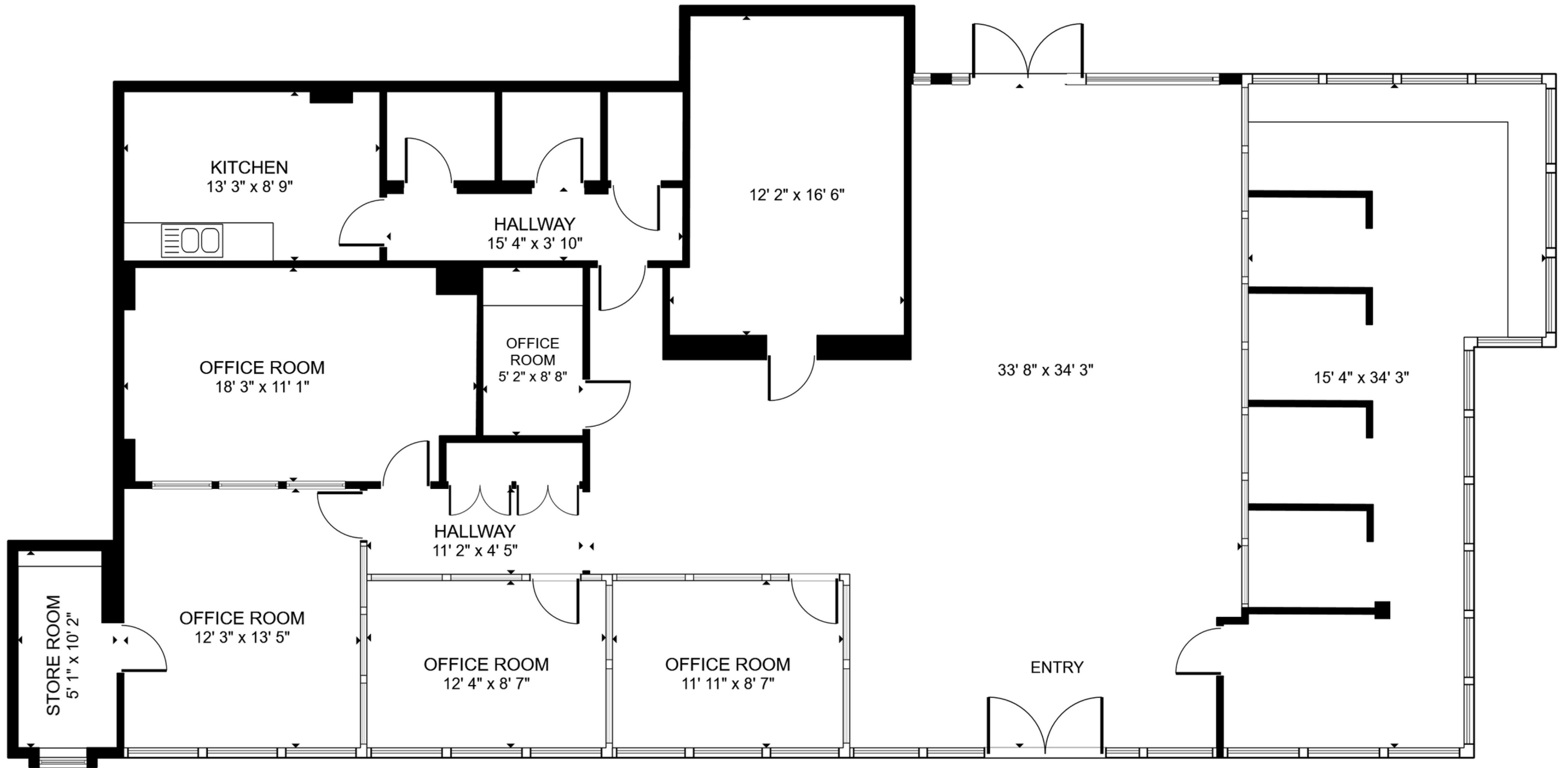
FLOOR PLAN
