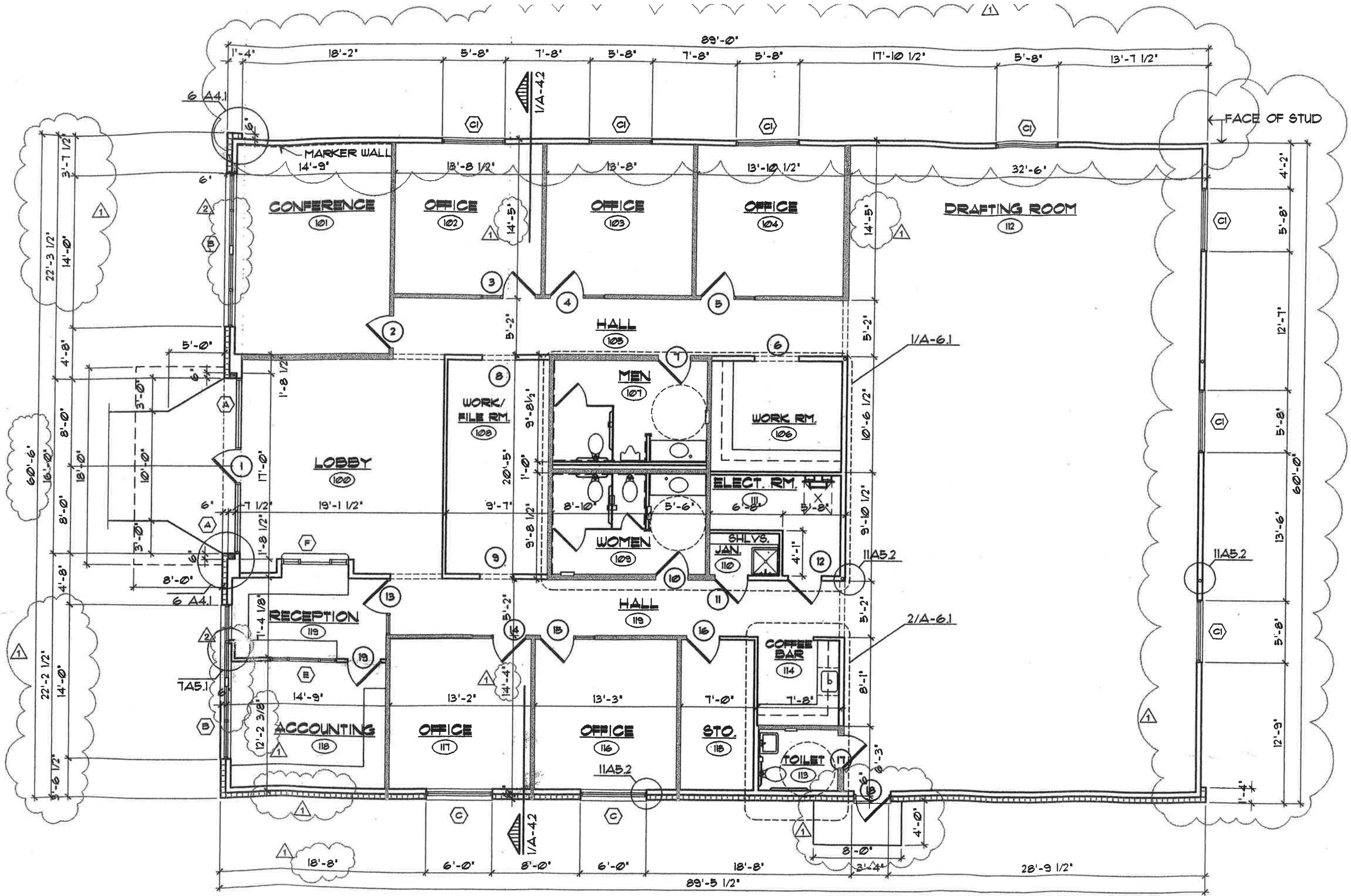
1 FLOOR PLAN
