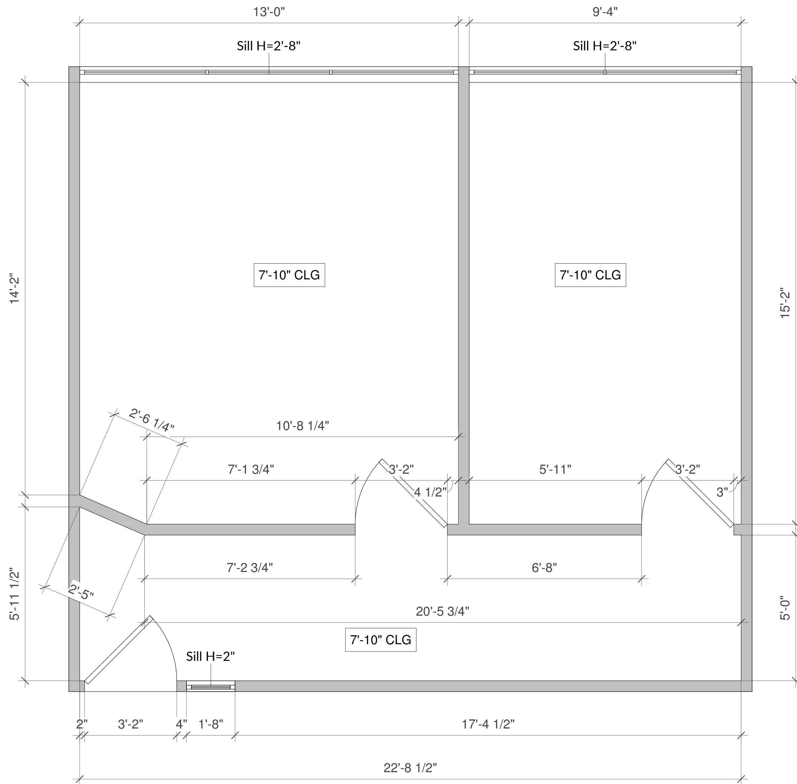
1 Floor Plan 1/2" = 1'-0"
