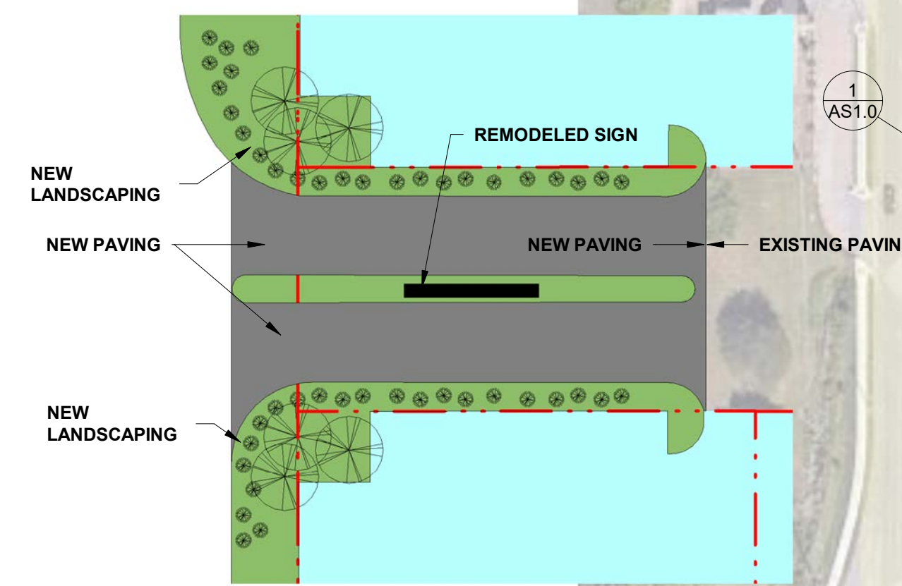
1 ENLARGED - SITE PLAN - ENTRY 1" = 40'-0"
