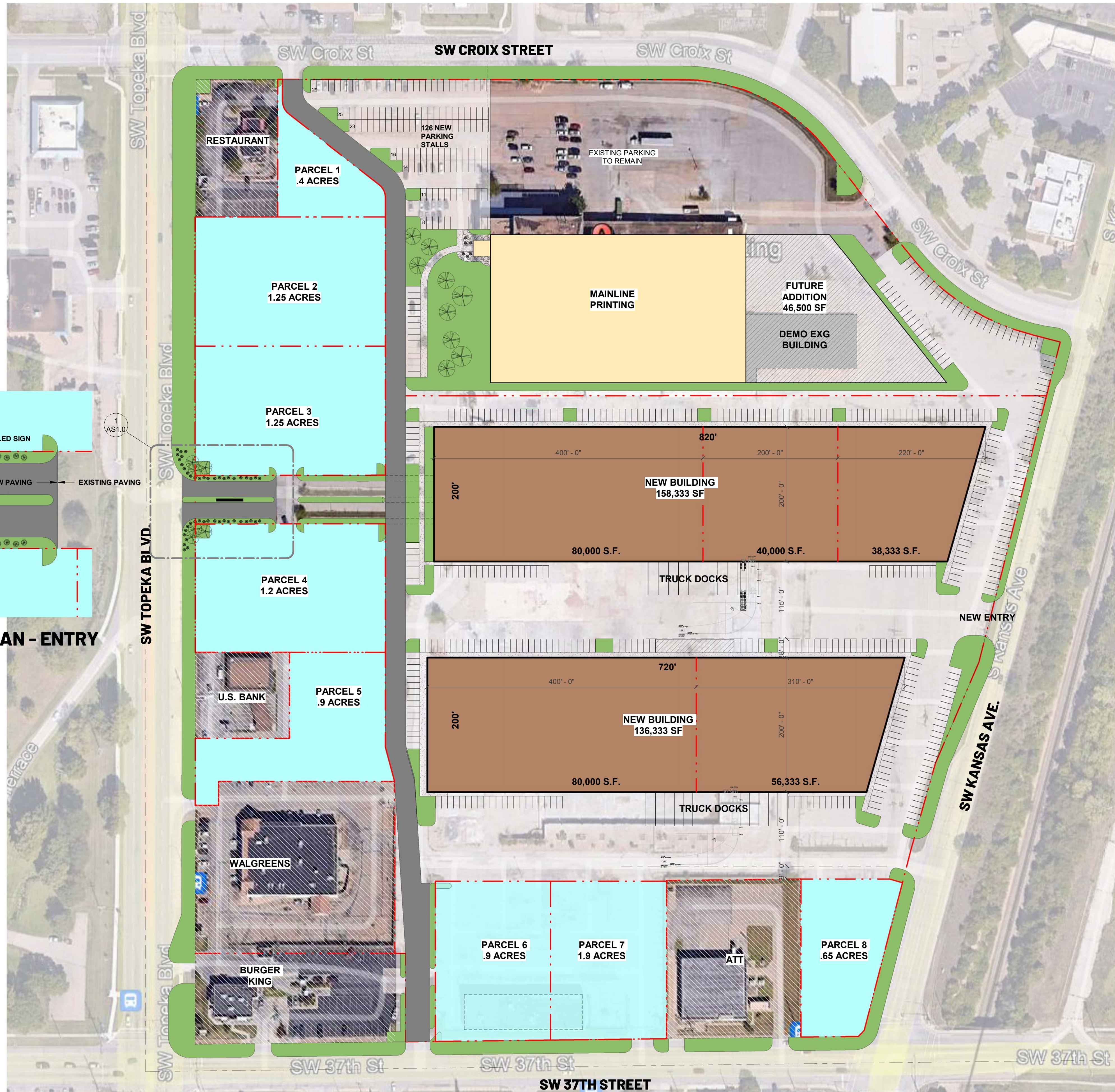
A ARCHITECTURAL SITE PLAN 1" = 80'-0" 0' 40' 80' 160'
