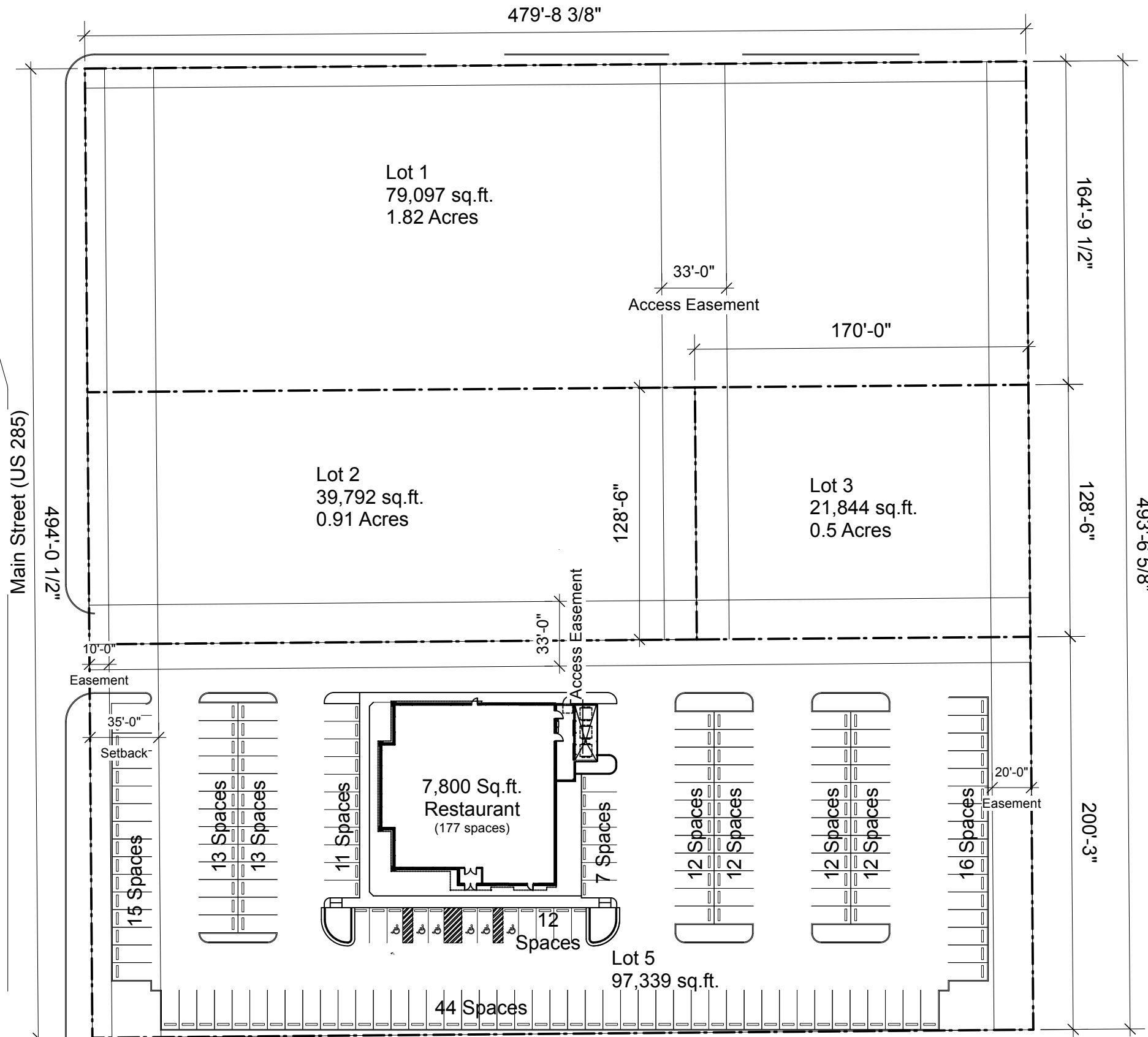
1 Site Plan 2.7 Acre Scale: 1:720
