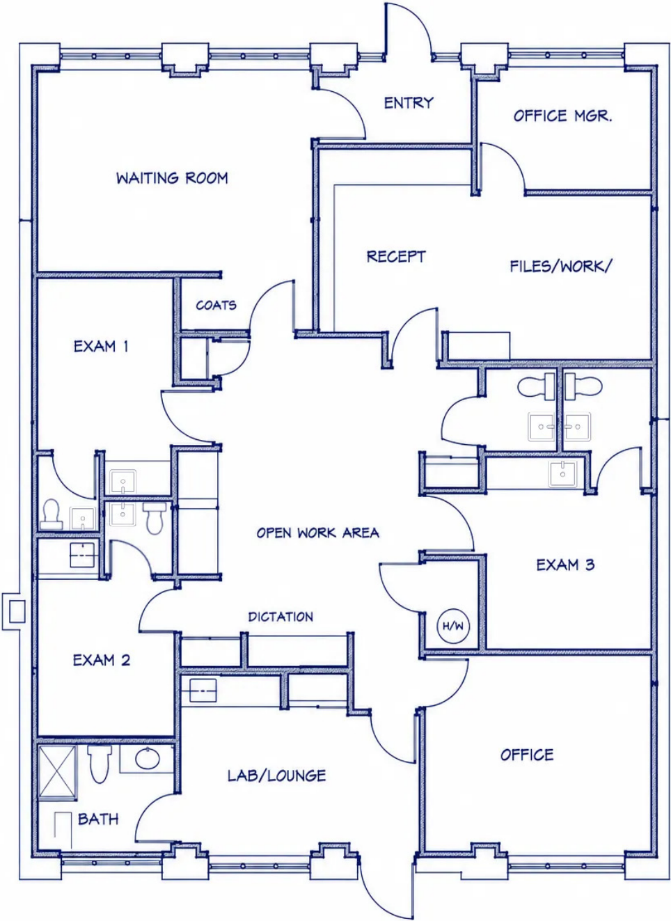
FLOOR PLAN
