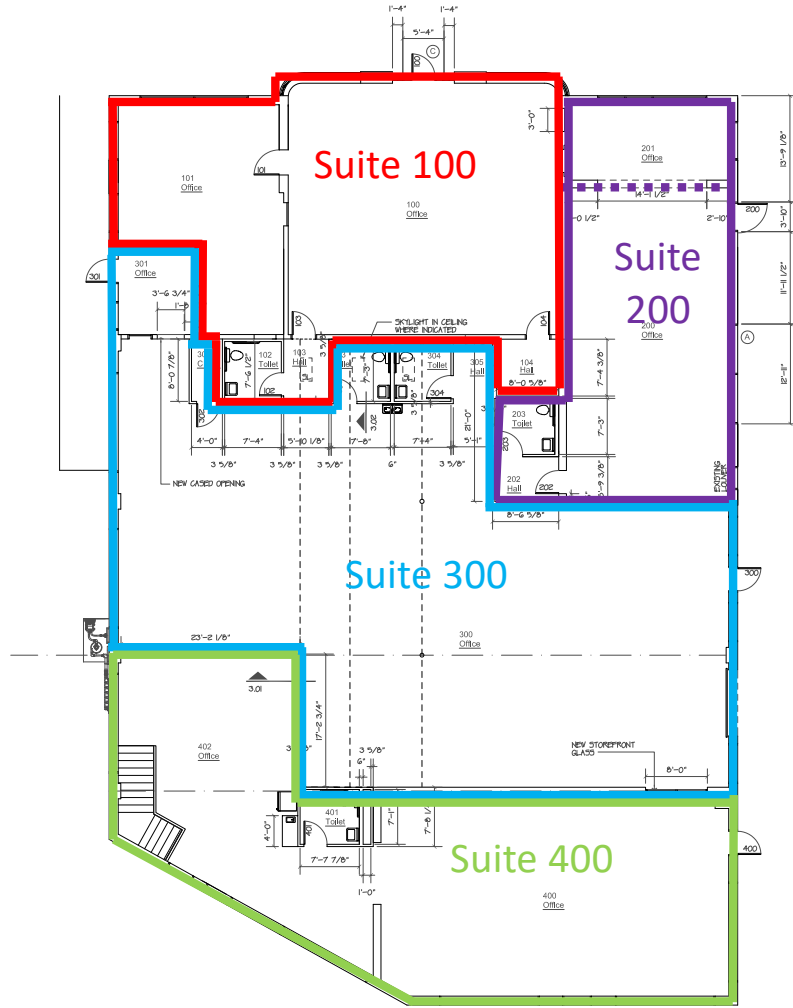
2.01 First Floor Plan SCALE 1/8" = 1'-0"
