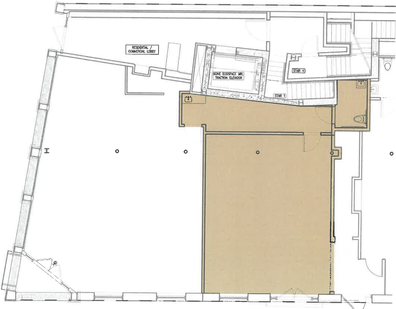
175 MOTT A GROUND FLOOR PLAN
