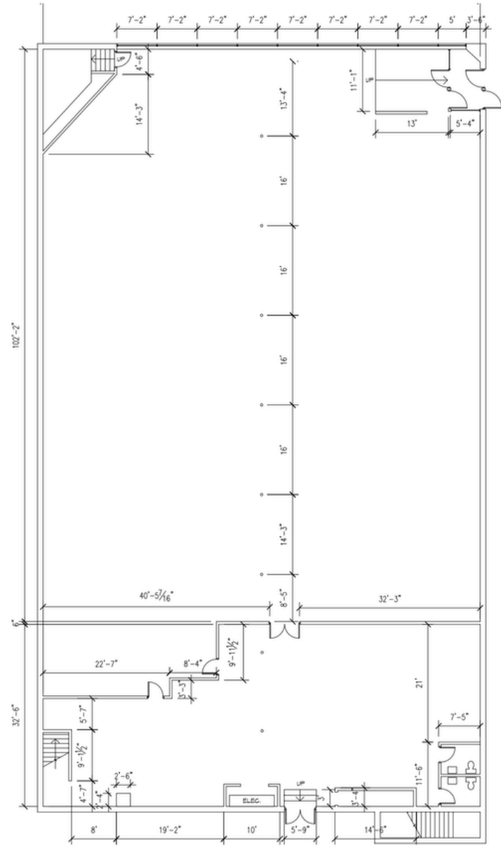
1 FIRST FLOOR PLAN S1 1/8" = 1'-0" PLAN NORTH
