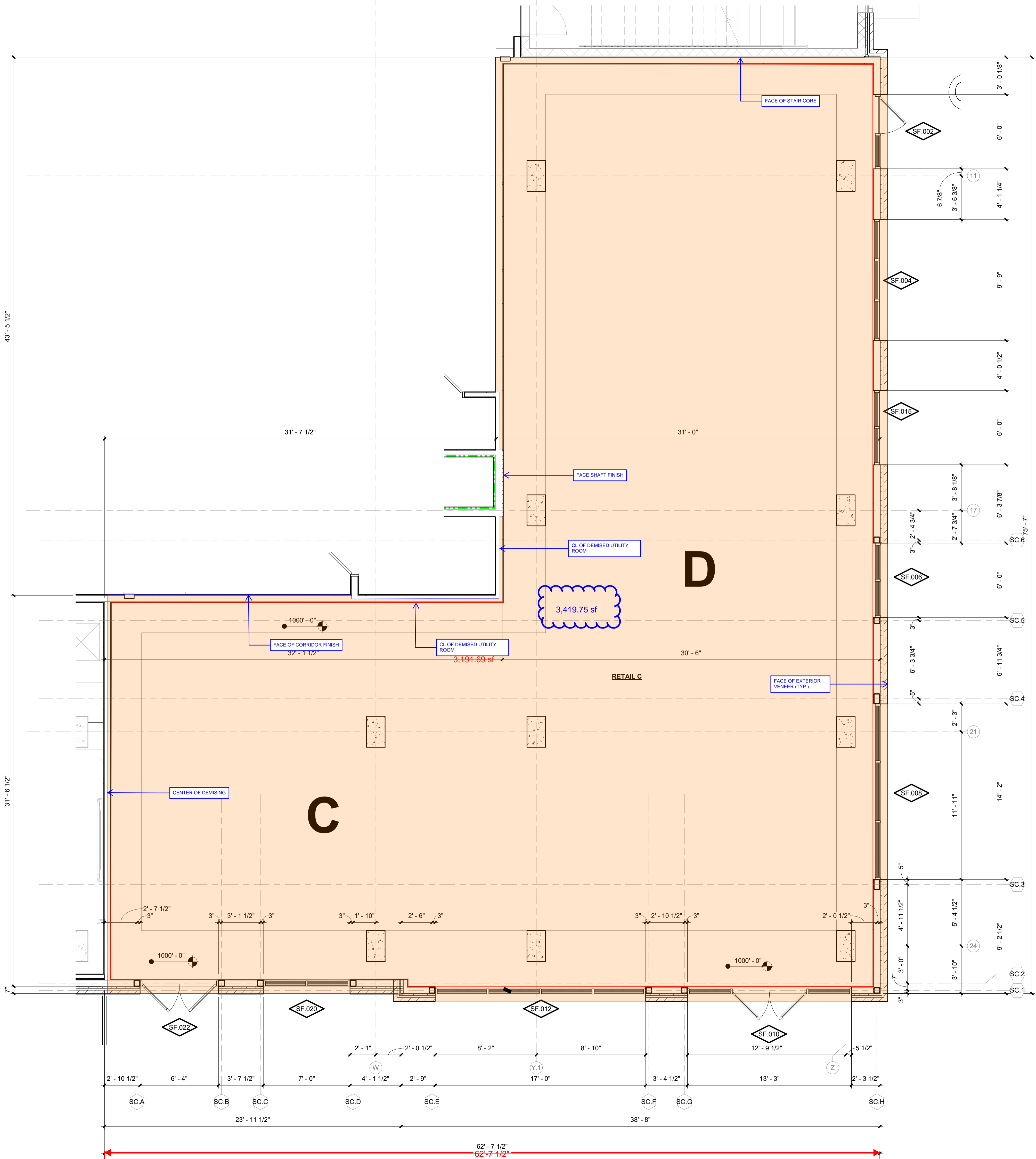
1 BLDG 3000 - RETAIL C ENLARGED PLAN - LEVEL 1000' - 0" 1/4" = 1'-0"
