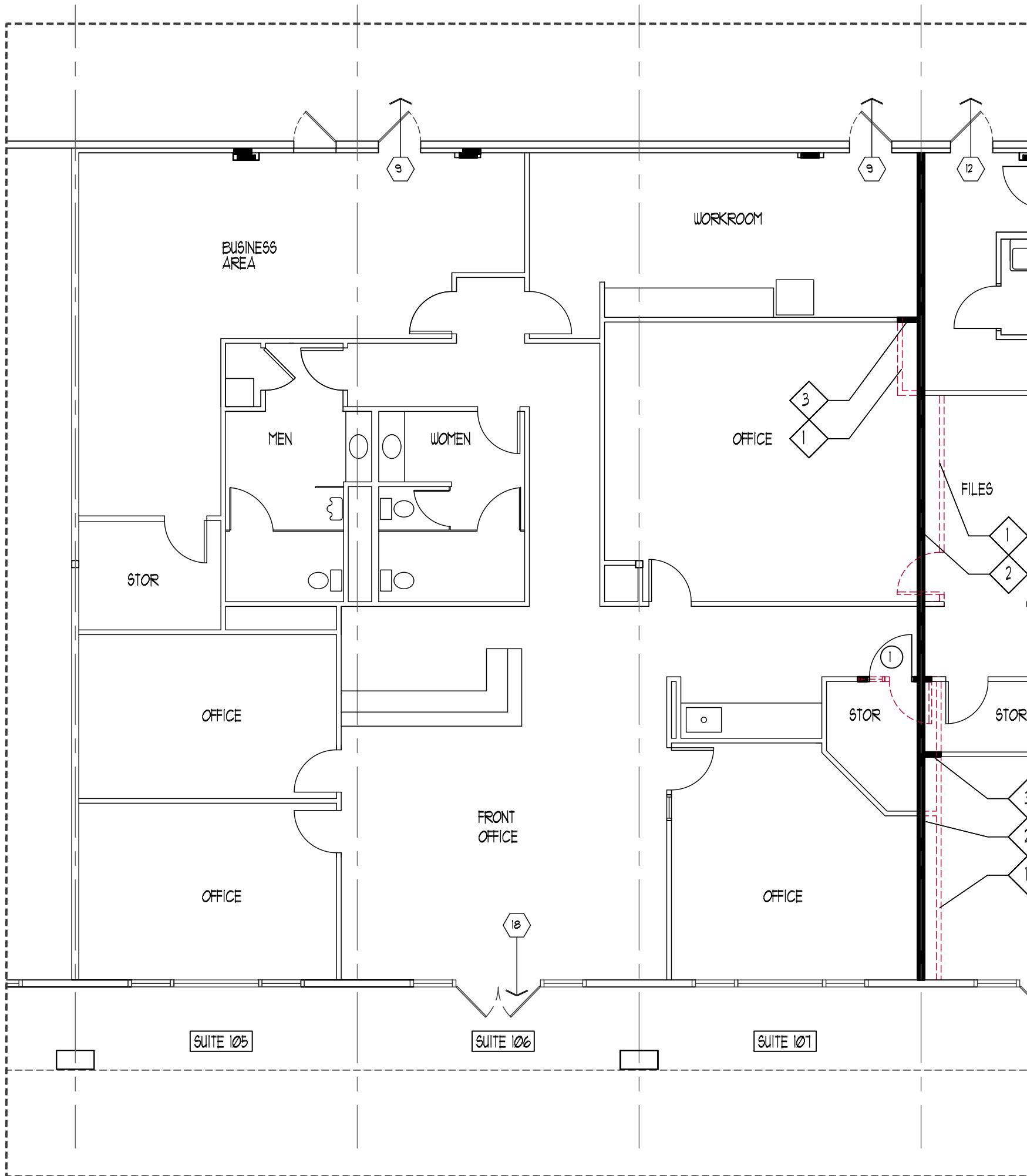
1 FLOOR PLAN
