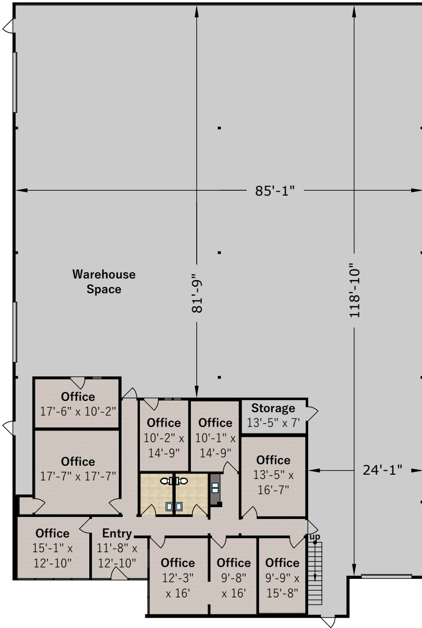
Office Space approx. 2,488 sqft
