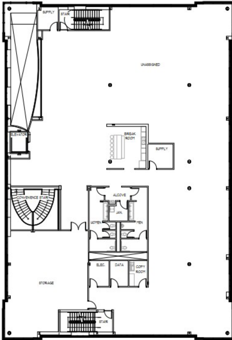
1 SECOND FLOOR EXISTING PLAN A-3 SCALE: 1/16" = 1'-0"
