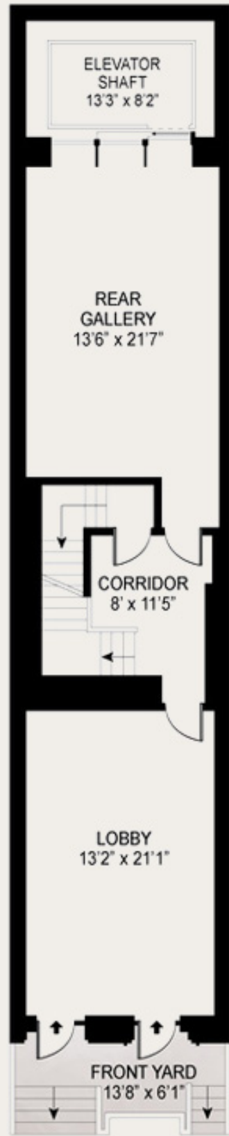
GROUND FLOOR
