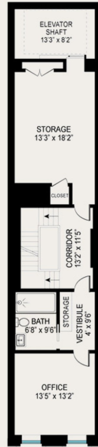
FOURTH FLOOR
