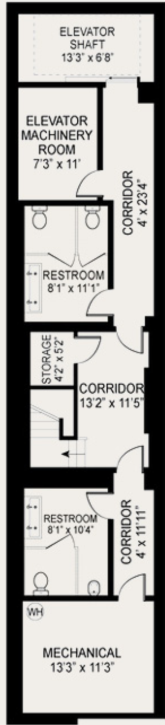
CELLAR FLOOR
