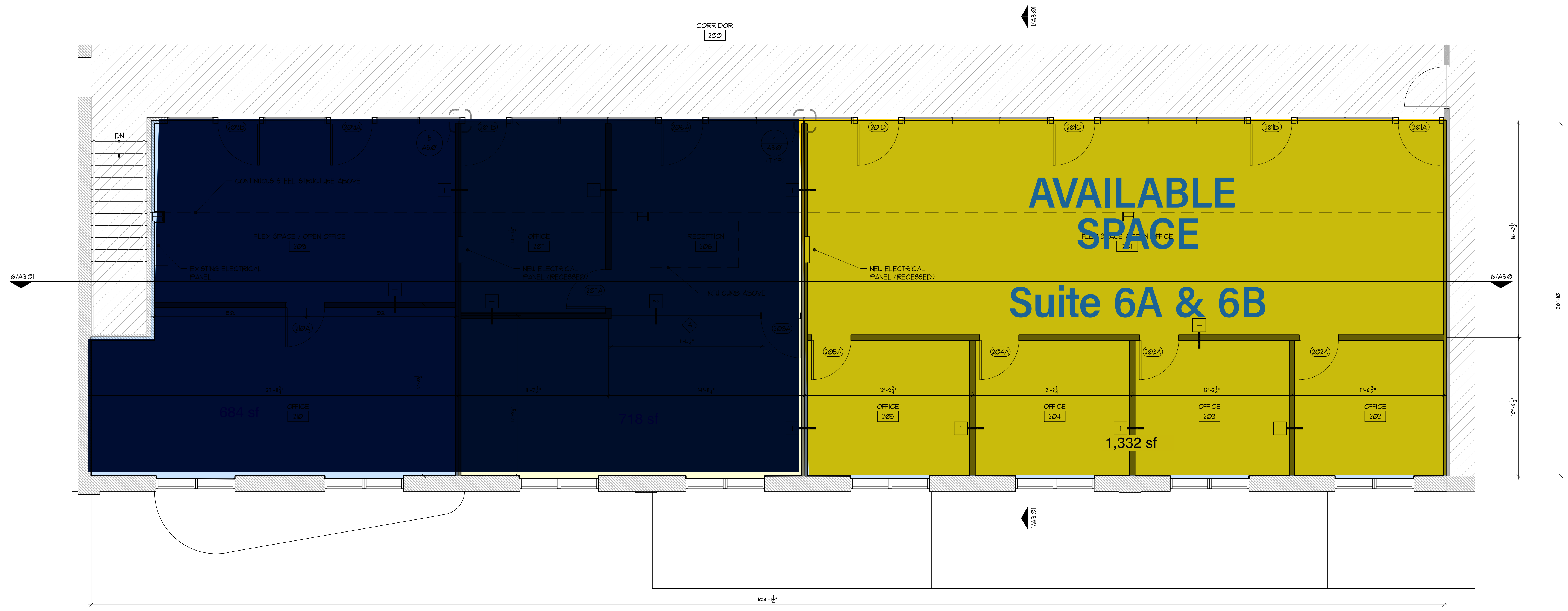
1 SECOND FLOOR PLAN A1.01 SCALE: 1/4"=1'-0"
