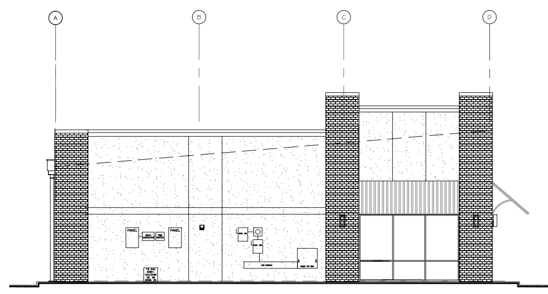
LEFT ELEVATION BLDG 2 & 3
