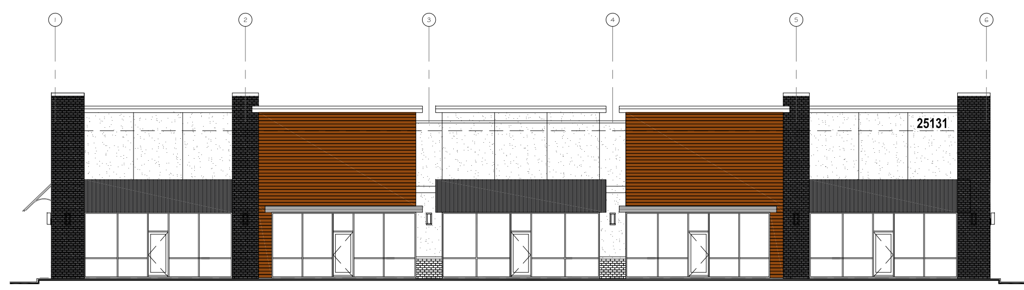
FRONT ELEVATION BLDG 2 & 3
