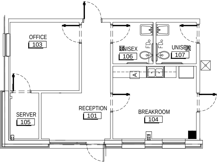
OFFICE FLOOR PLAN | BUILDING 5 AND 6
