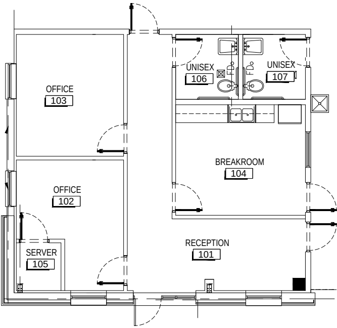
OFFICE FLOOR PLAN | BUILDING 7 AND 8
