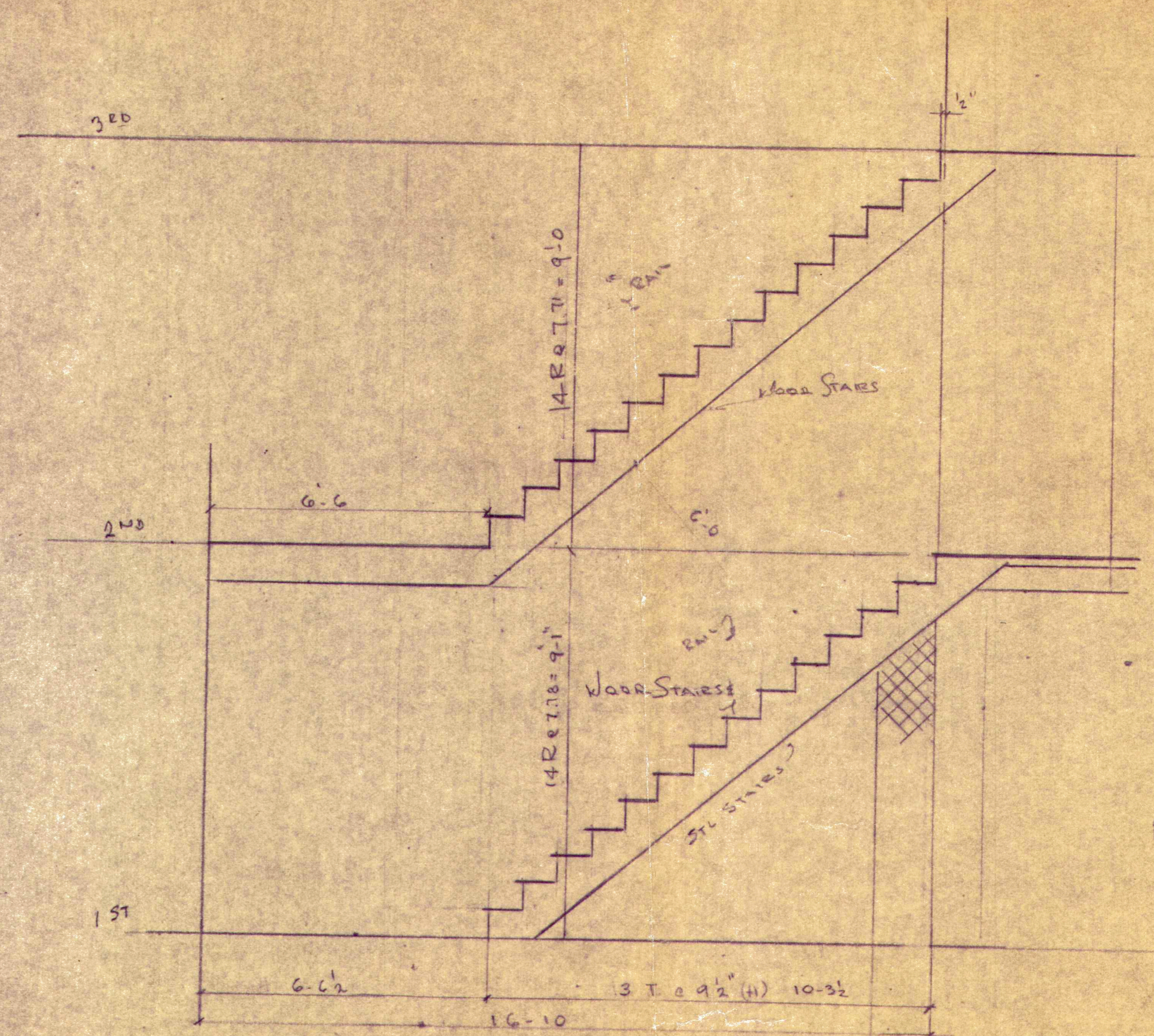
SECTION 2 3/8-11-0
