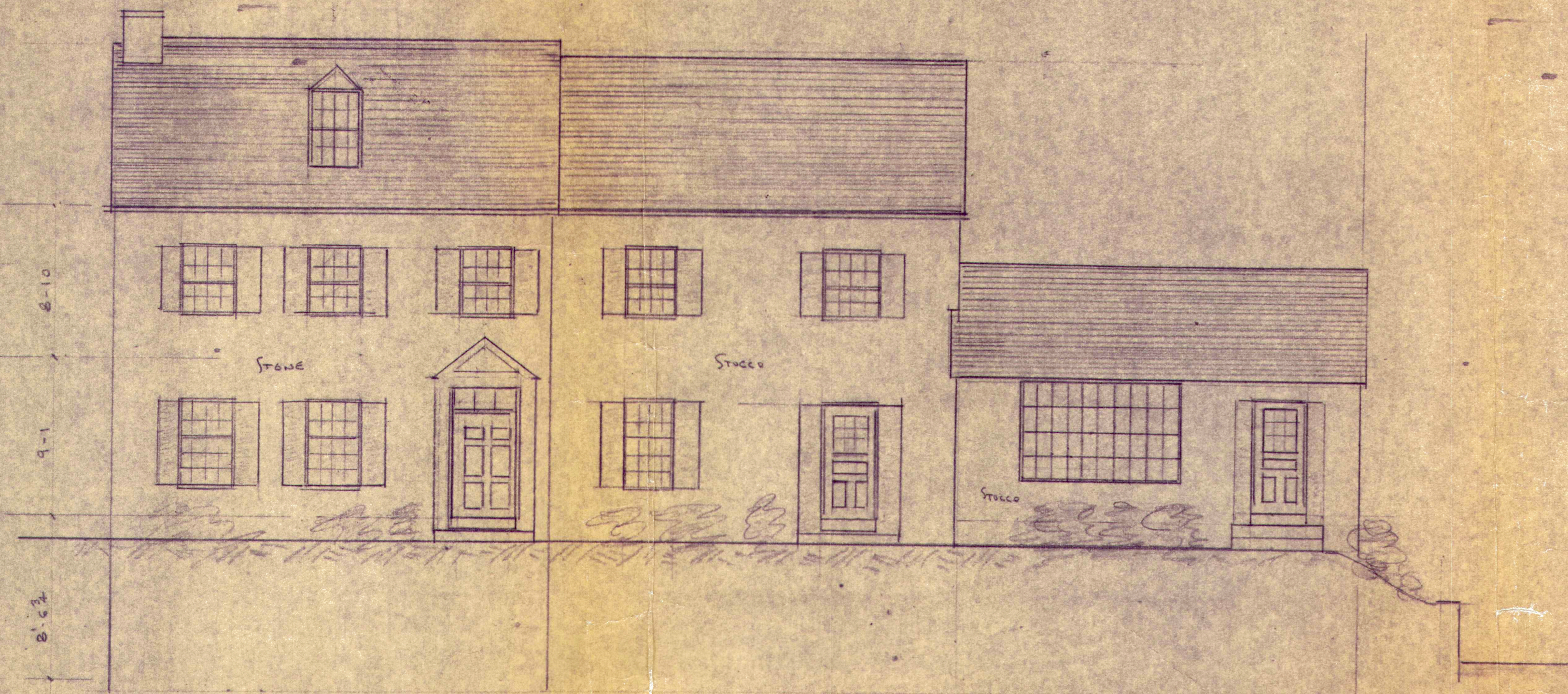
ELEVATION 1 3/6-11-0
