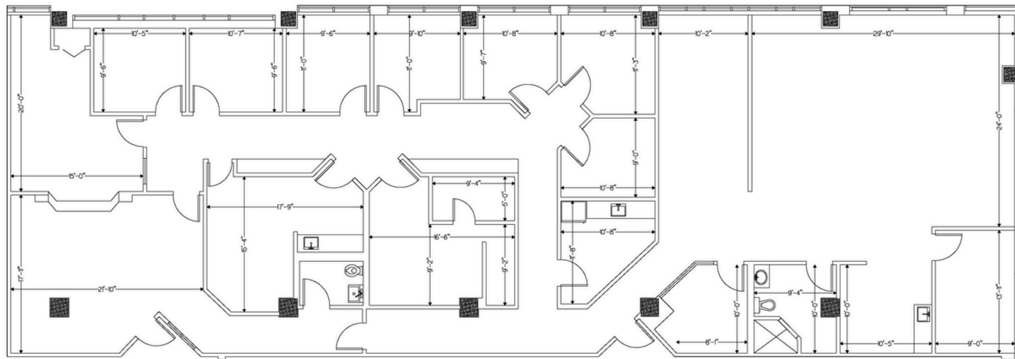
BUILDING PLAN
