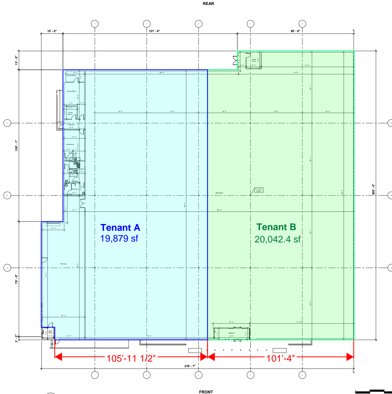
A1 MAIN FLOOR
