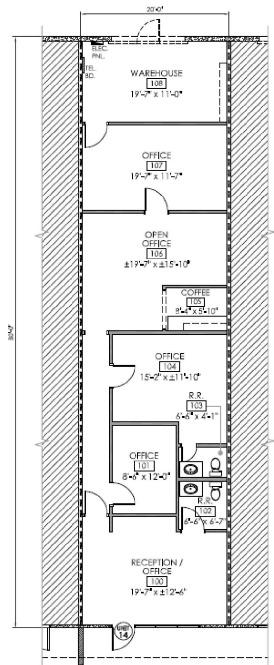
FLOOR PLAN SCALE: 1"=10'-0"
