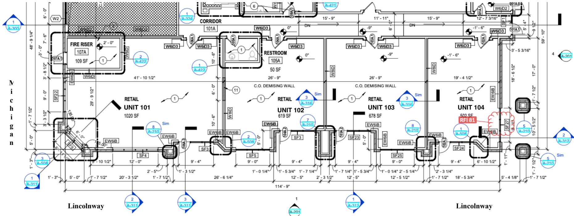
1 BUILDING A - FIRST FLOOR PLAN 1/8" = 1'-0"
