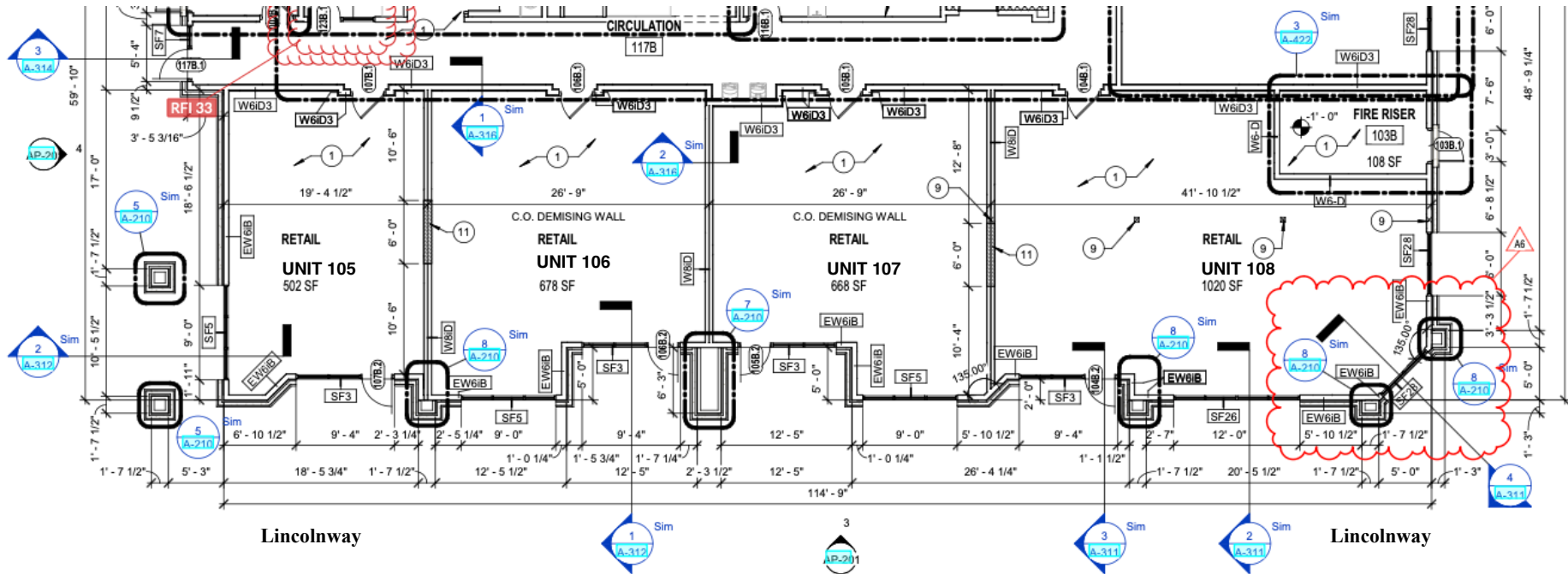
1 BUILDING B - FIRST FLOOR PLAN 1/8" = 1'-0"
