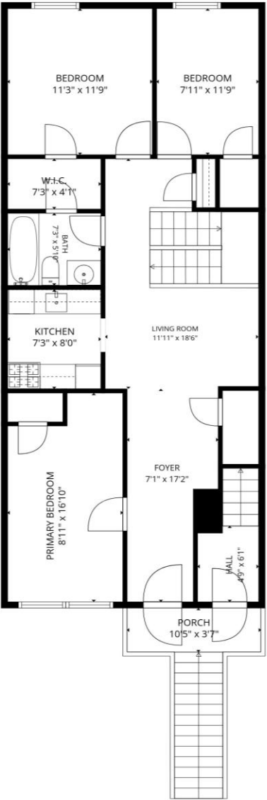
2nd floor
