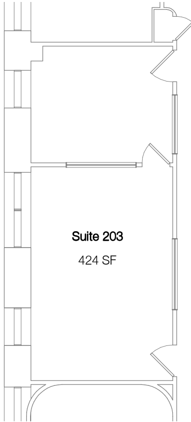
① Suite 203 1/8" = 1'-0"
