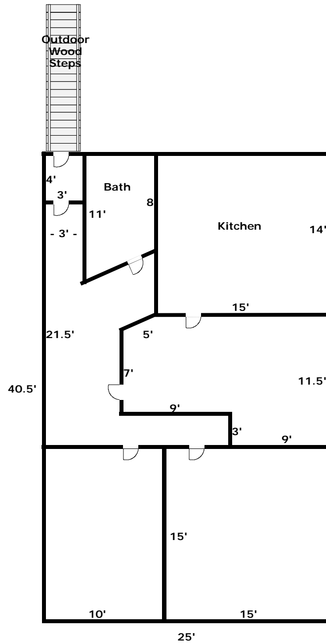
901 S. COLORADO, SALEM, VA SECOND FLOOR - 1,012+/- SF
