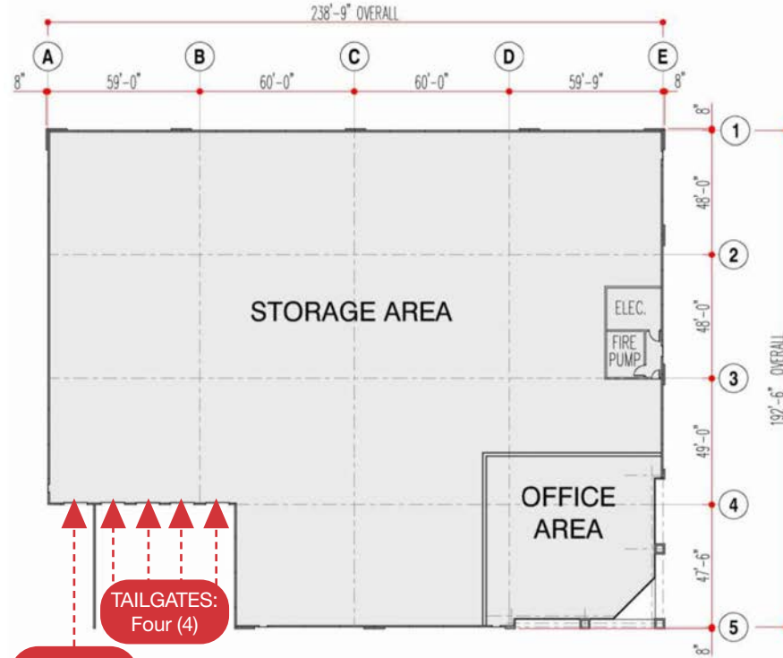
① GROUND FLOOR PLAN
