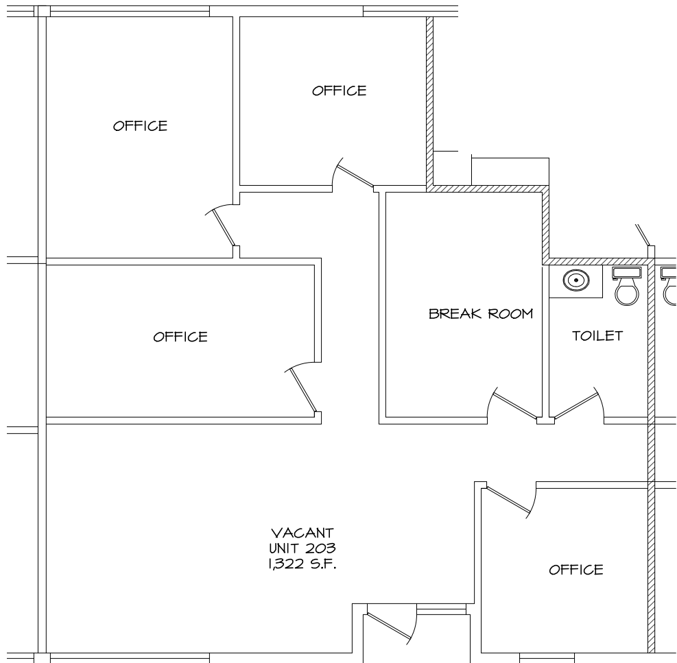
① UNIT 203 - EXISTING FLOOR PLAN SCALE: 1/8" = 1'-0" 1,322 TOTAL SQUARE FEET
