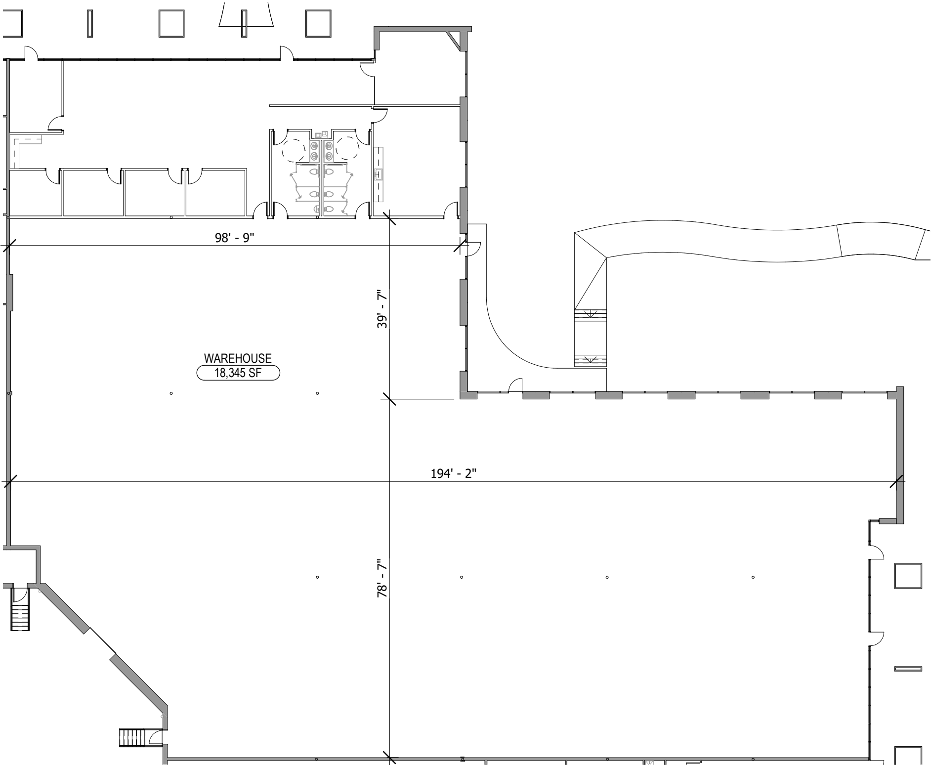
WAREHOUSE PLAN
