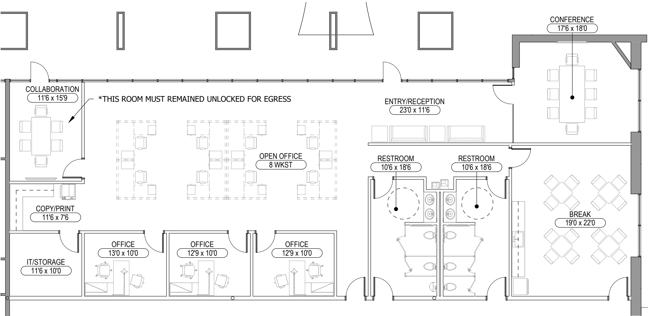
OFFICE PLAN
