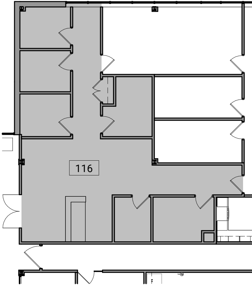
2 Suite 116 - Partial Level 1 Existing Floor Plan 3/32" = 1'-0" 4' 8' 12'
