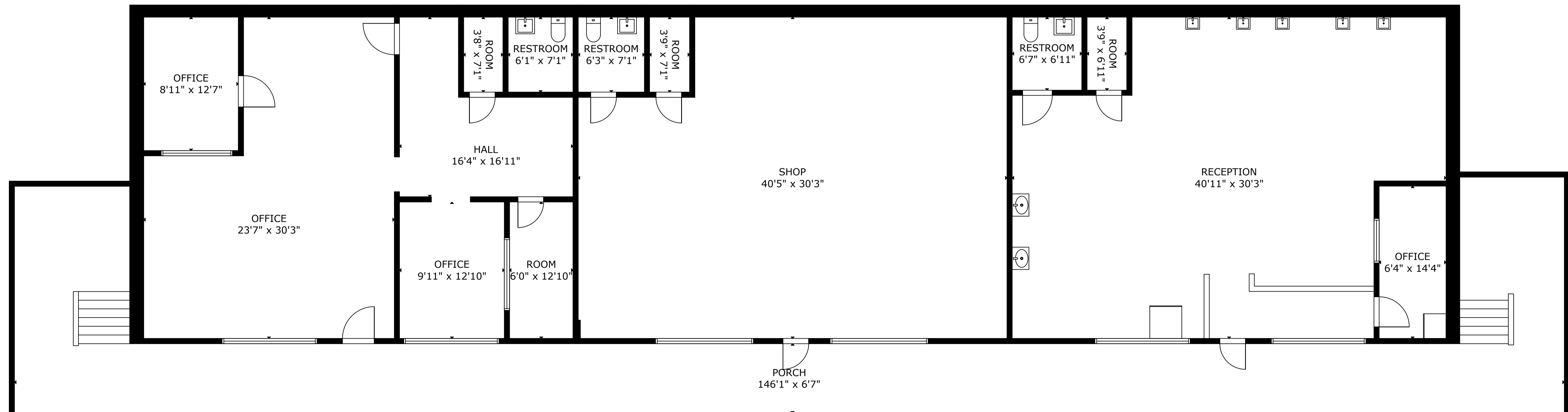
MAIN FLOOR
