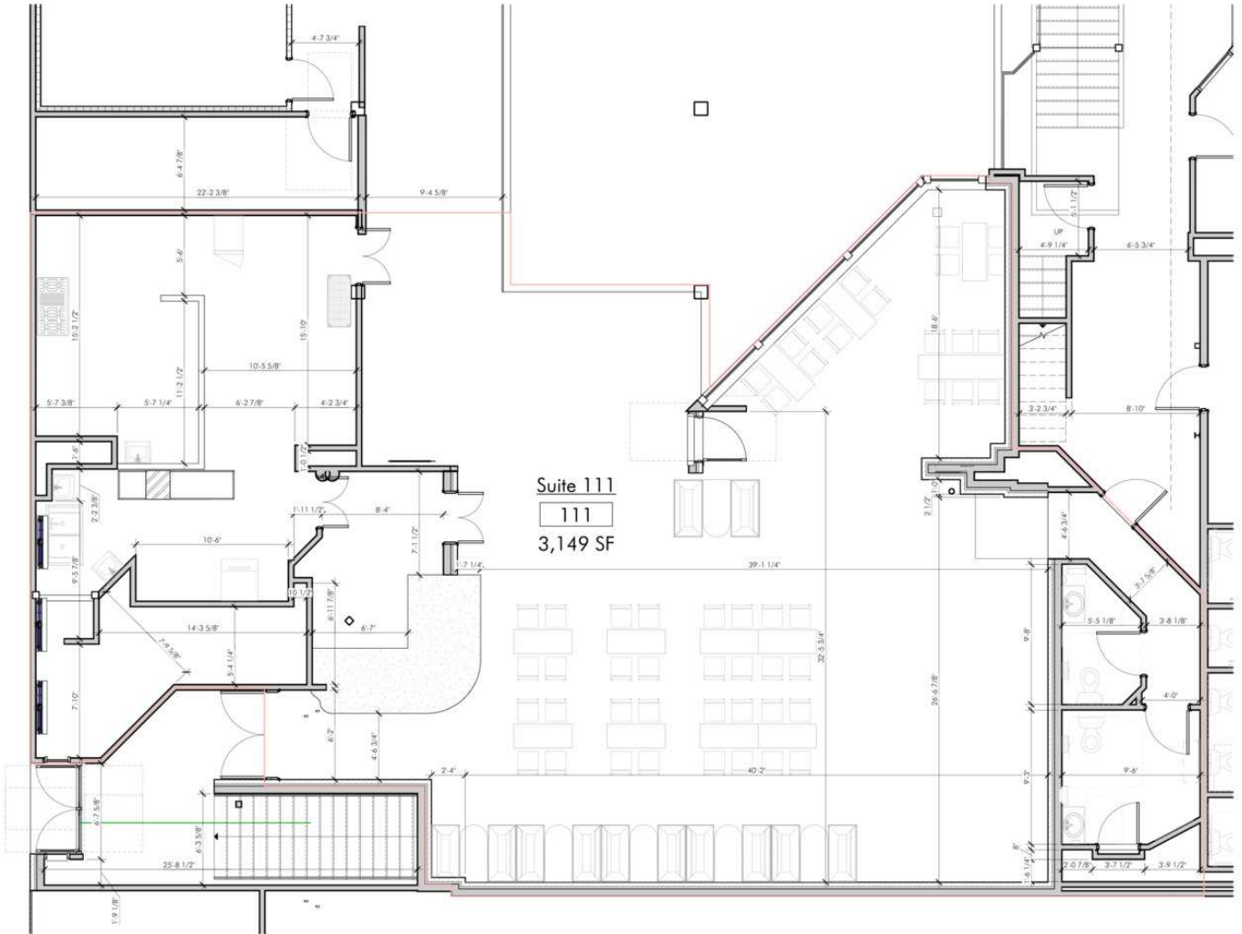
1 SUITE 111-FLOOR PLAN 1/4" = 1'-0"
