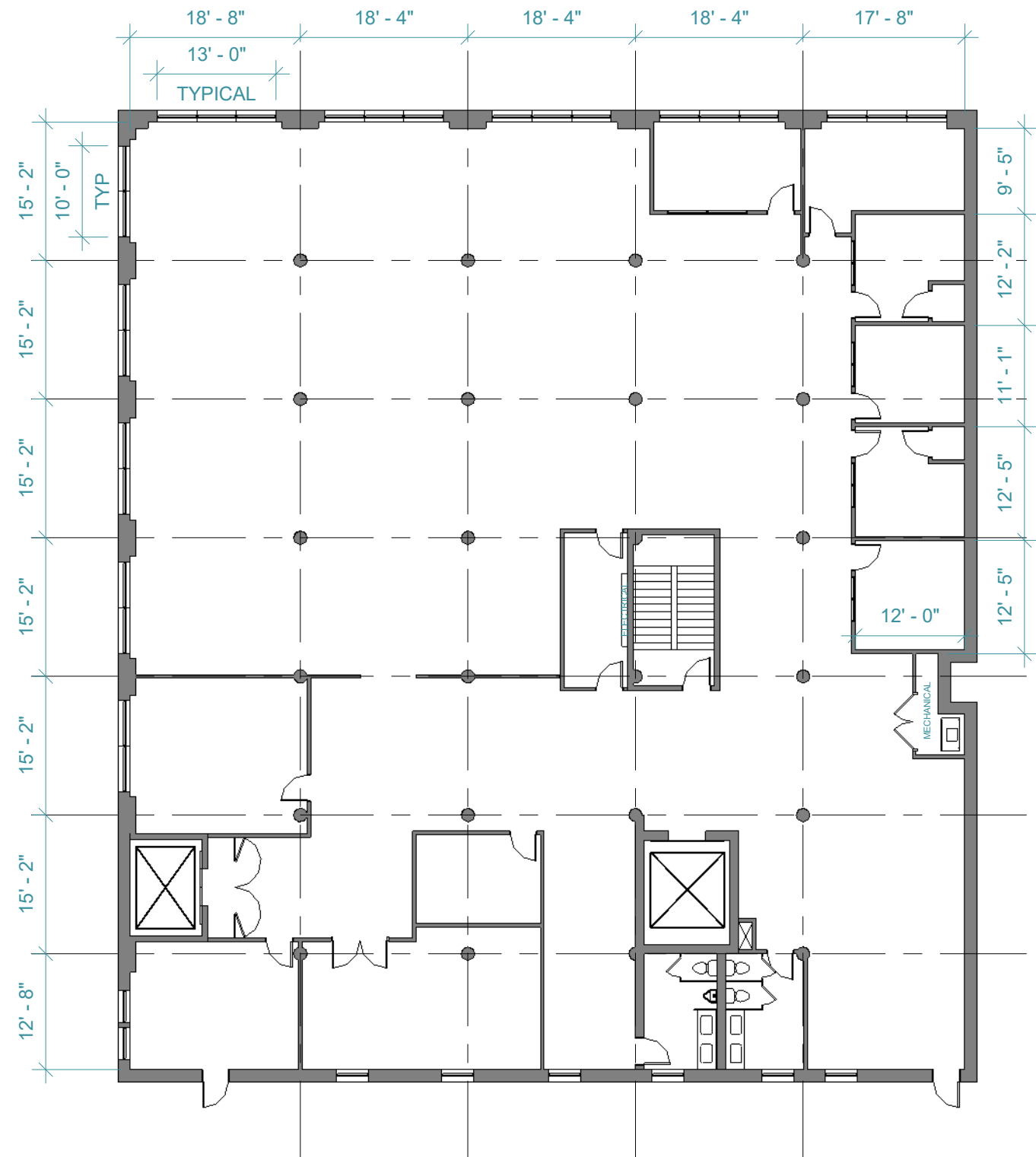
5TH FLOOR EXISTING PLAN
