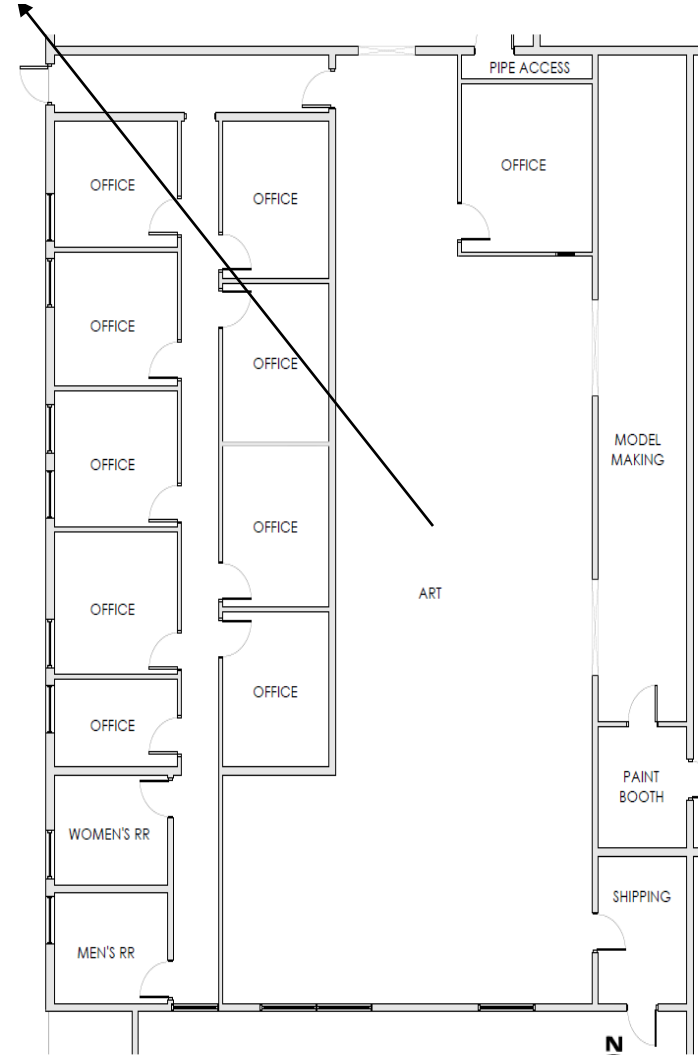
2 EXISTING ENLARGED ART DEPARTMENT FLOOR PLAN A2.0 1/8" = 1'-0"
