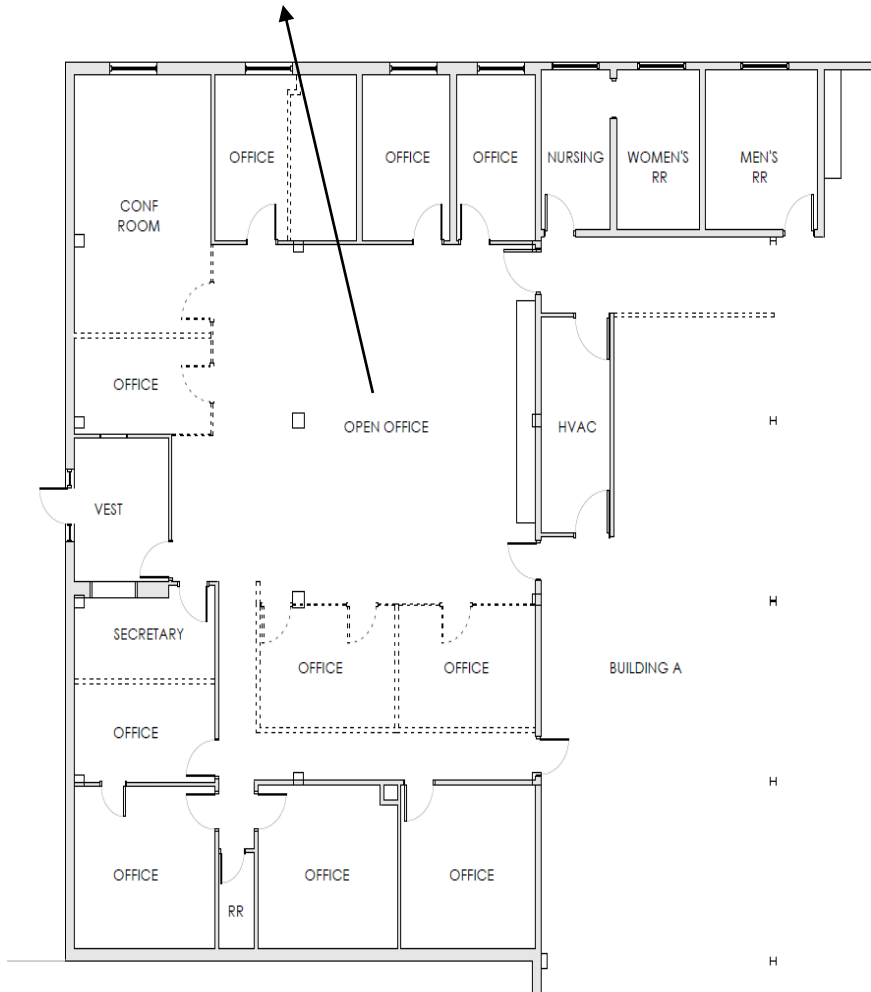
1 EXISTING ENLARGED OFFICE FLOOR PLAN A2.0 1/8" = 1'-0"
