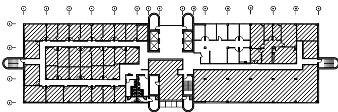
2ND FLOOR - LOCATION KEY PLAN
