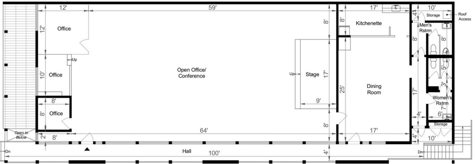
FLOOR PLAN
