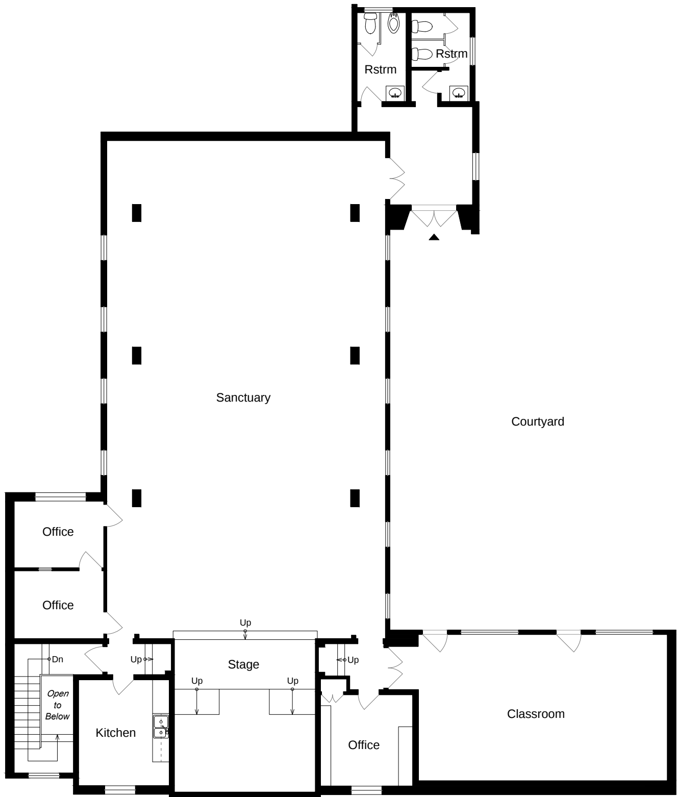
FIRST FLOOR
