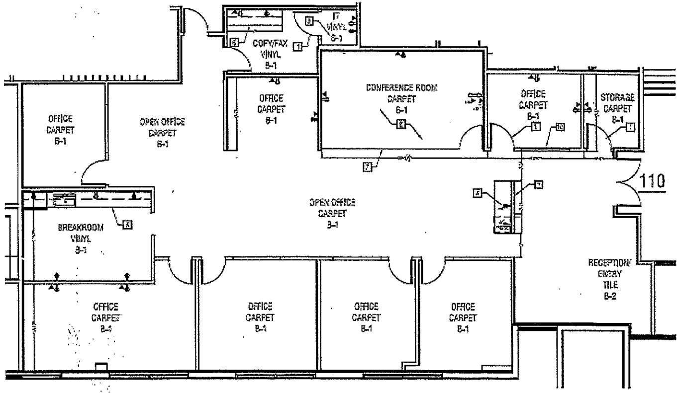
2 FLOOR PLAN scale: 3/16" = 1'-0"
