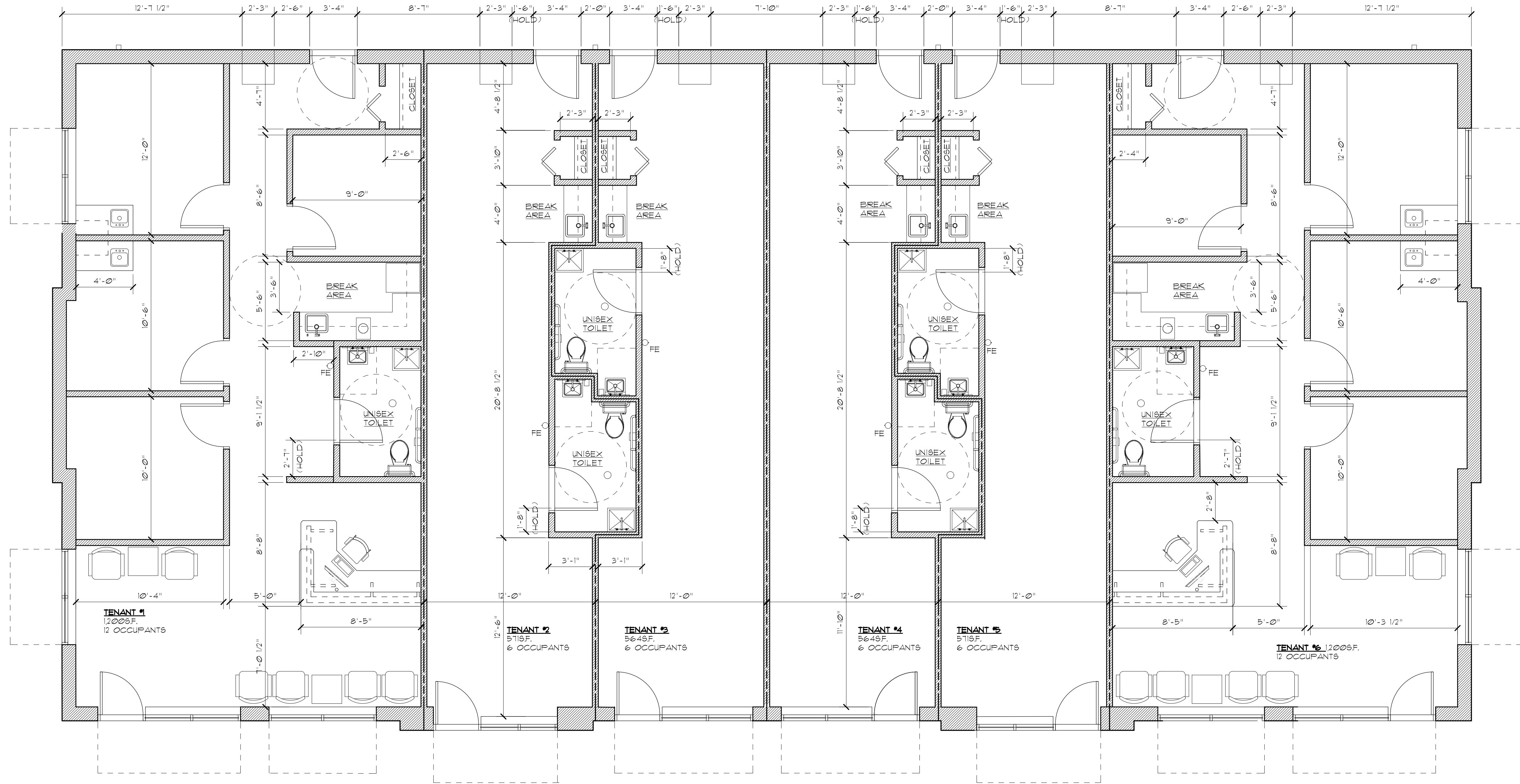
FLOOR PLAN INTERIOR WALL DIMENSIONS SCALE: 1/4"=1'-0" NORTH
