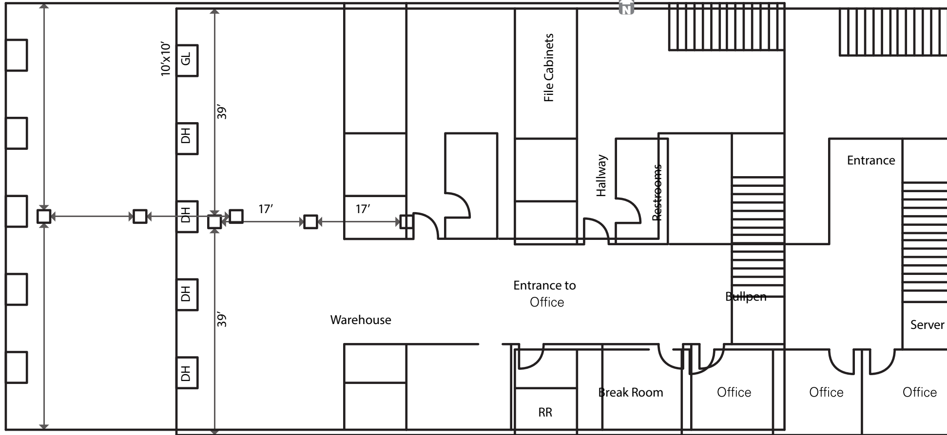
MAIN FLOOR
